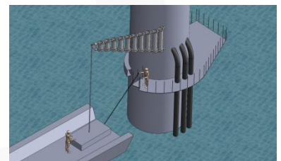
Fig. 1: Vessel is safely in boat landing.
