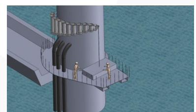
Fig. 4: Placing of equipment.
